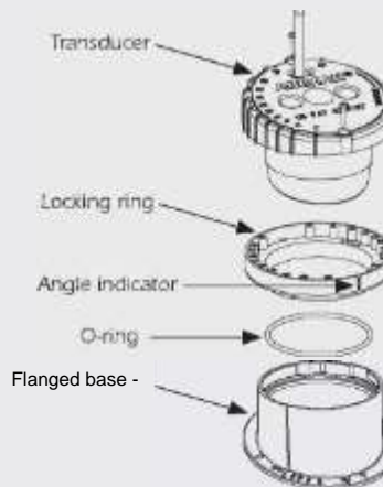
P79 Transducer
