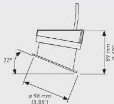
Dimensions at Maximum Installation Angle
